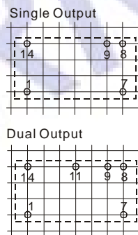
FOOTPRINT DETAILS
